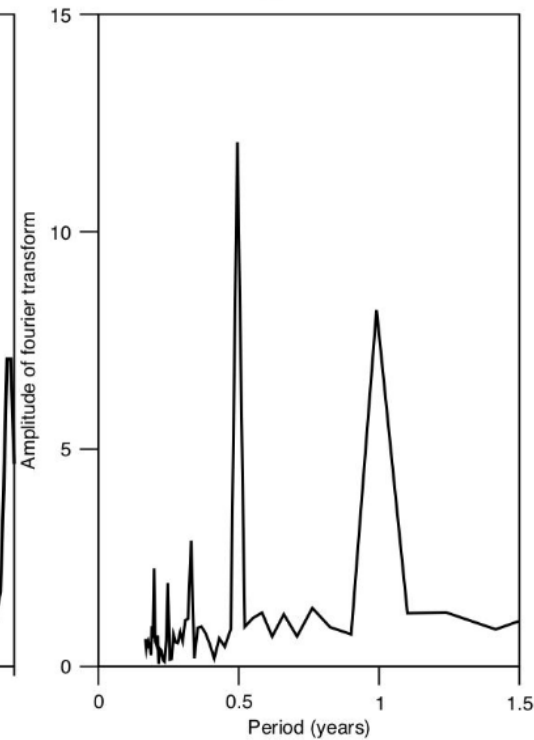
Fourier transform of Google trends
