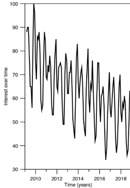
Google trends of Fourier Transform
